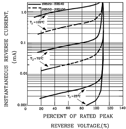
FIG.4-TYPICAL REVERSE CHARACTERISTICS
