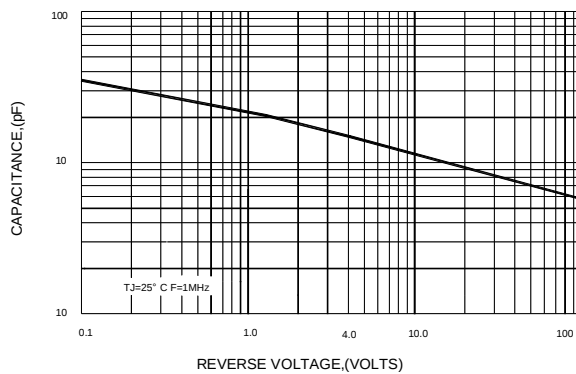
FIG.5-TYPICAL JUNCTION CAPACITANCE
